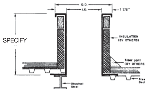
RC-6A STYLE- VERTICAL NAILER
